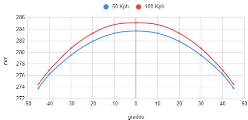
ROLLING RADIUS - Front
