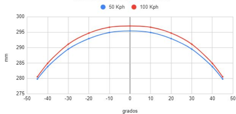
ROLLING RADIUS - Rear
